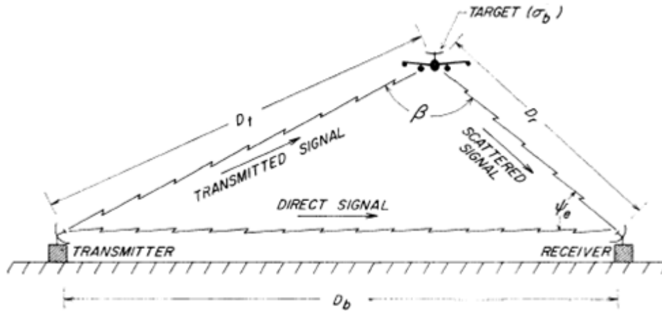
Fig. 1: Bistatic Radar [8]
